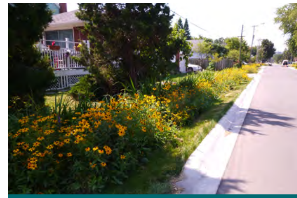
Figure 4.3.8: Boulevard units installed in Mississauga as part of an upgrade from a rural cross section. (Source: CVC)
