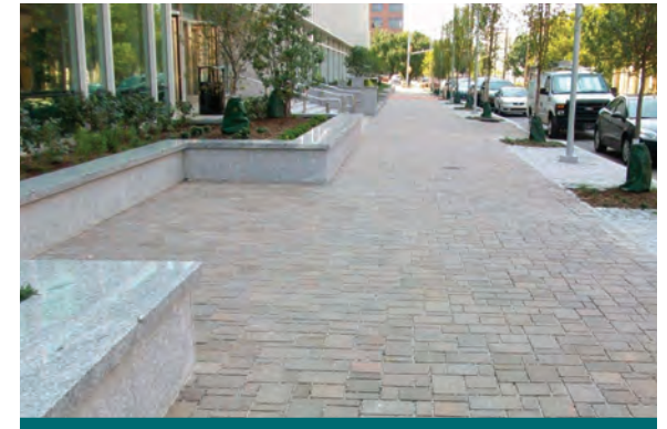
Figure 4.3.24: Permeable paver sidewalk along a minor arterial in Raleigh, NC. (Source: Fred Adams Paving )
