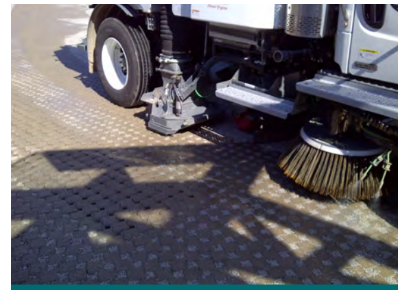
Figure 10.2.2: Vacuum sweepers will remove accumulated debris between pavers, but can also remove aggregate from paver joint (note the voids behind the sweeper truck.) Always replenish any lost joint aggregate following vacuum sweeping. (Source: Aquafor Beech)
